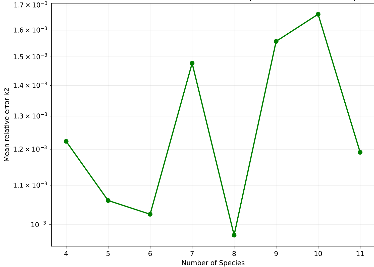
30, 30, 30 — Mean relative error k2 vs number of species (zoomed: 4 to 11 species)
